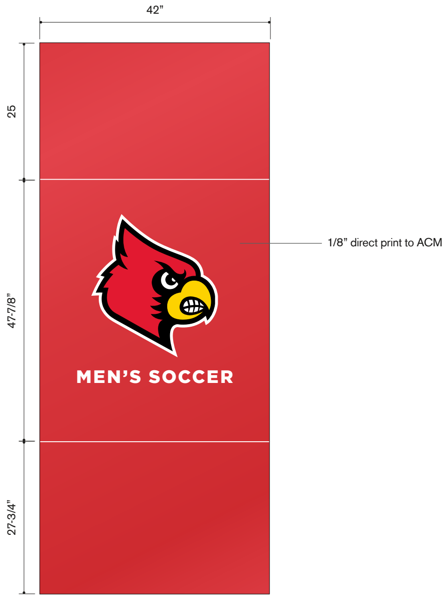
DIMENSIONAL PLAQUE
