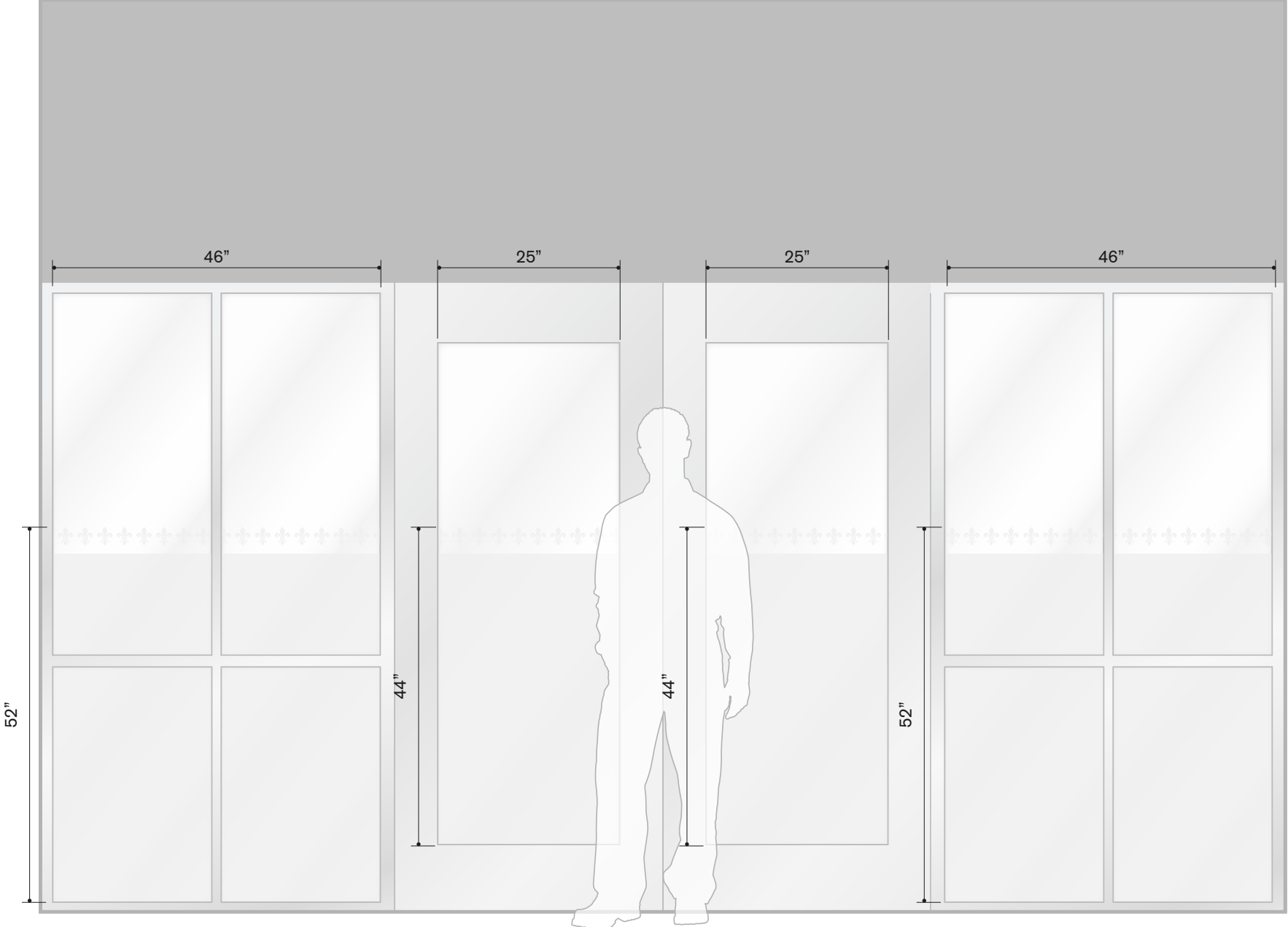
ETCH MARK CONTOUR CUT VINYL
