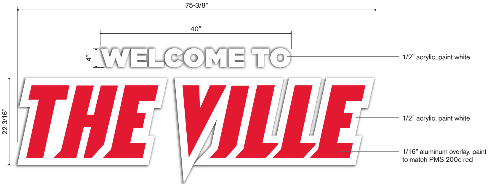
DIMENSIONAL LETTERING/LOGO
