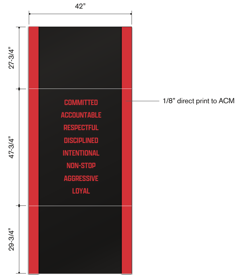
WALL PLAQUE
