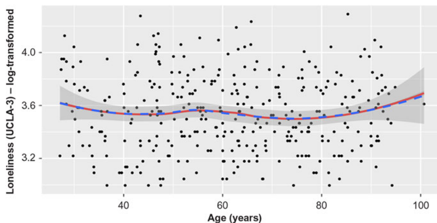
Figure 1. Relationship between Loneliness severity and Age ( N = 340 ). Blue dotted line: LOESS curve fit. Red solid line: Linear spline model using age 53 year knot/break point. UCLA-3 = UCLA Loneliness Scale (Version 3); measure of loneliness (Russell, 1996). The linear spline model significantly differs from linear age effect (Wald statistic = 7.93, p = 0.019 ).
