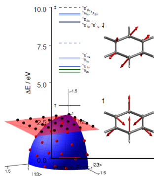
CONCEPT Different Orbitals For Different Electron Configurations to Develop New Methods of Computational Simulation
