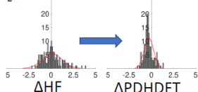
DEVELOPMENT Simulating Excited States with Difference Projected DFT For Excited States
